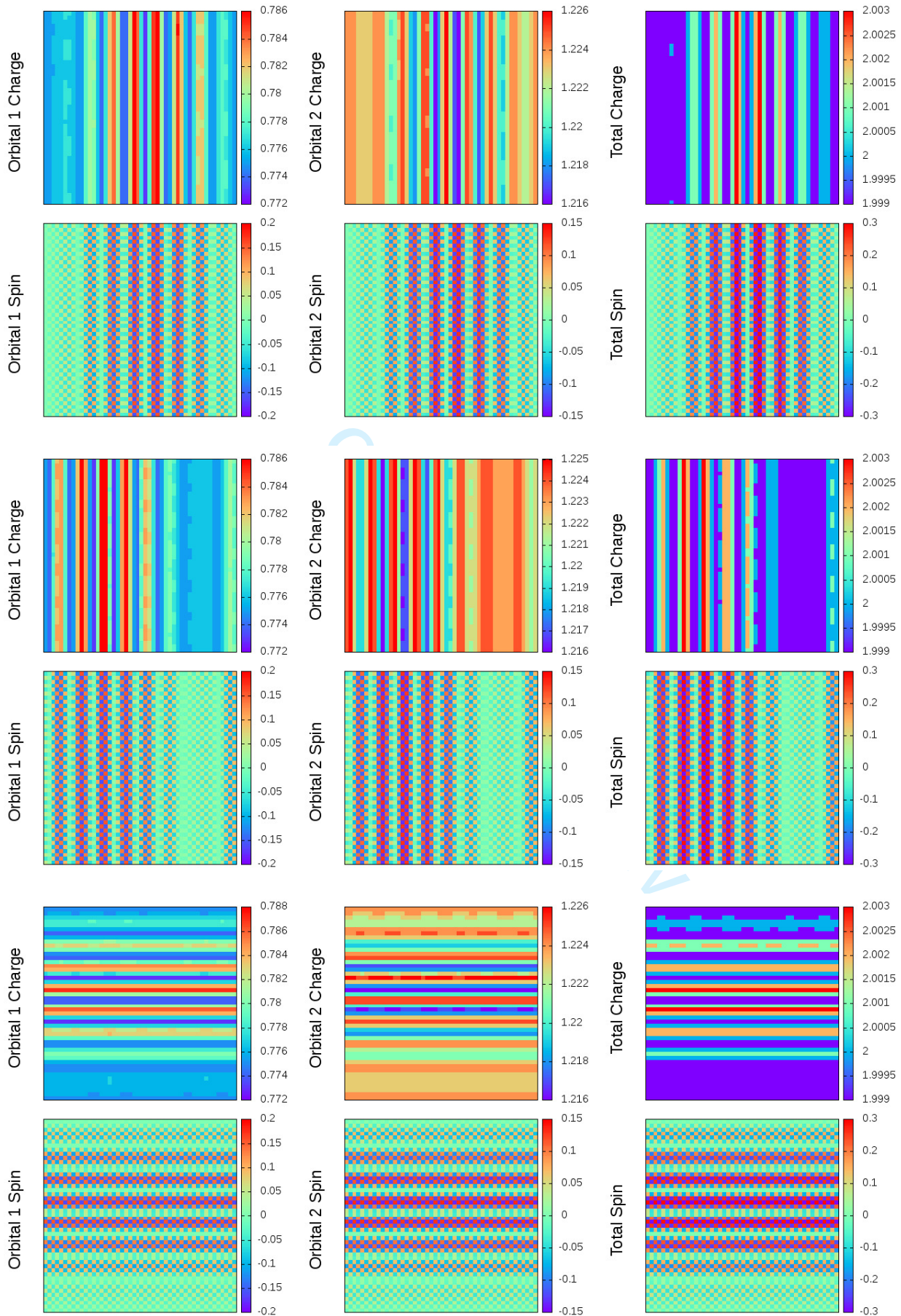
Figure 5: Three examples of the stripe type of ground state for polarization P=0.8 . Each example consists of six panels, three above for charge and three below for spin. The colorbar provides the amplitudes.
