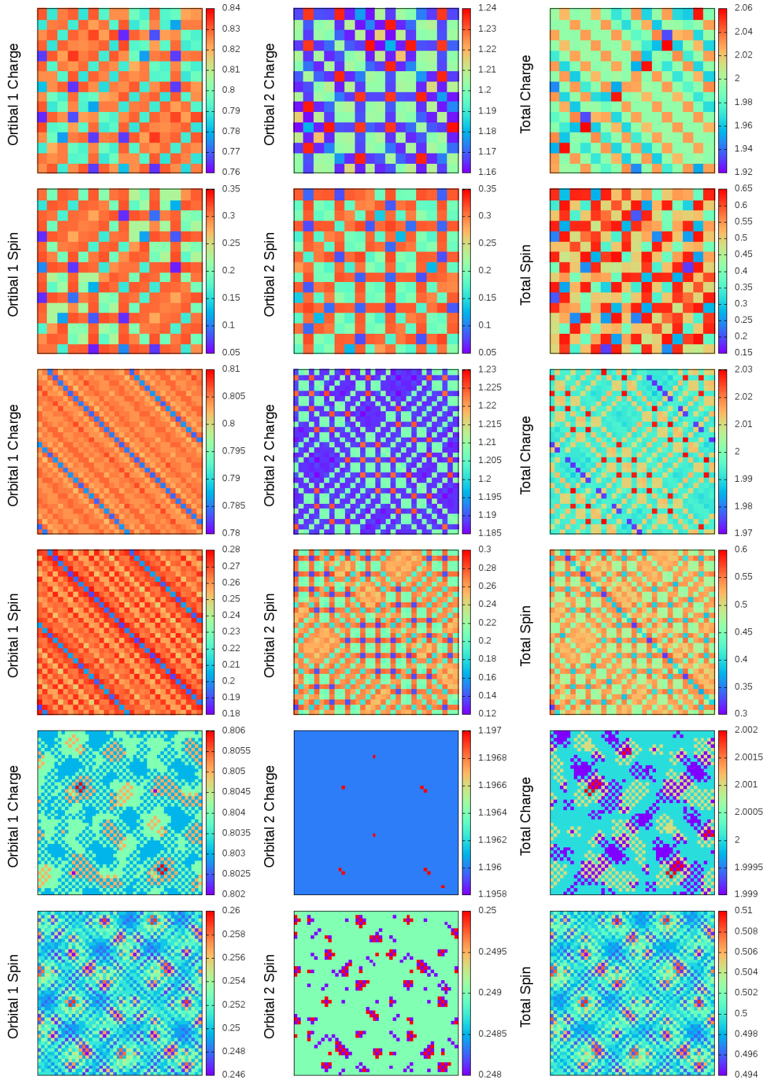
FIG. 3. Charge and spin density arrays for polarization P=1/4 , run #2, arranged as in Fig. 2.
