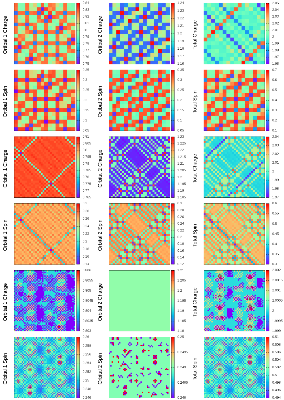
FIG. 2. Charge and spin density arrays for polarization P=1/4 , run #1. The top six panels are for N=16 , charge arrays above spin arrays, and from left to right progressing from orbital 1 to orbital 2 to the total (their sum). The center six panels are for N=32 , the lower six panels are for N=48 .
