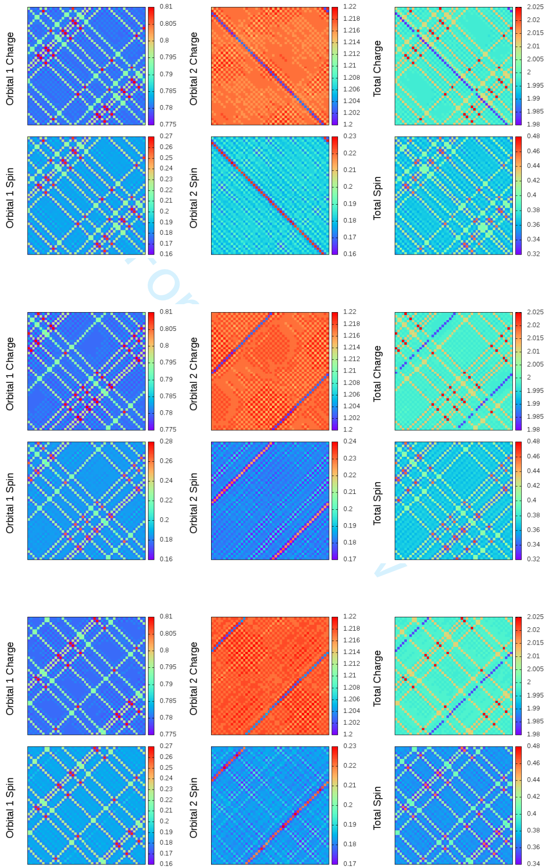
FIG. 6. Charge and spin density arrays for polarization P=3/16 , for three different cases (random starts) all for N=48 . For this polarization the spin variation remains for the largest lattice size and is very consistent for the different runs.
