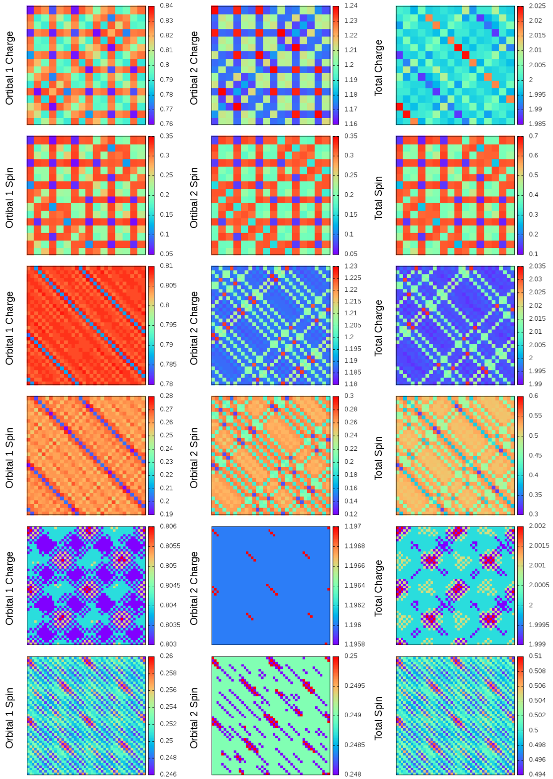
FIG. 5. Charge and spin density arrays for polarization P=1/4 , run #4, arranged as in Fig. 2.
