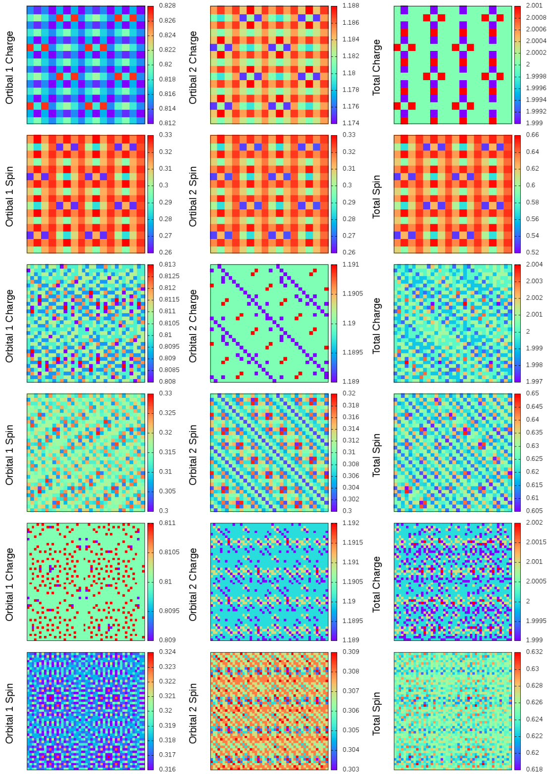
FIG. 7. Charge and spin density arrays for polarization P=5/16 , run #1, arranged as in Fig. 6.
