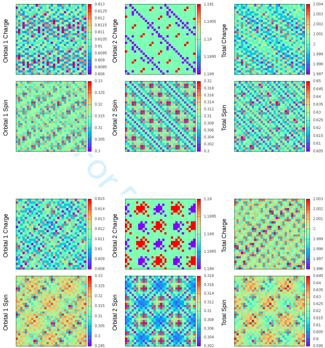
FIG. 1. Charge and spin density arrays for polarization P=5/16 , for two different runs and displaying N=32 only. There are six panels for each run, the set of six arranged as in the text and in following figures that include results for N=16, 32 , and 48 . The description in the text justifies why we classify these two results as showing no significant difference.
