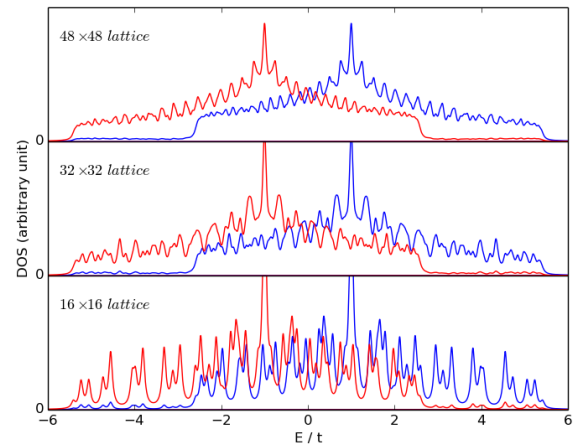
Figure 1: The non-interacting density of states for the N=16, 32, and 48 simulations cells, as labeled. The progression illustrates the relative sampling of states in energy for the three cases.
