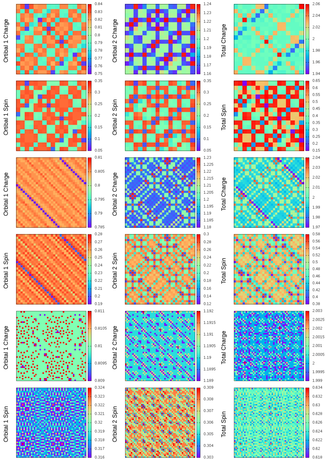
FIG. 4. Charge and spin density arrays for polarization P=1/4 , run #3, arranged as in Fig. 2.
