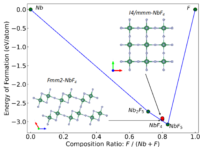
Figure 1. Convex hull of the Nb-F system at zero pressure and zero temperature. Insets show crystal structures of I4/mmm - NbF_4 and Fmm2 - NbF_4 . Calculations were done using VASP code [11] with the PBE exchange-correlation functional.
