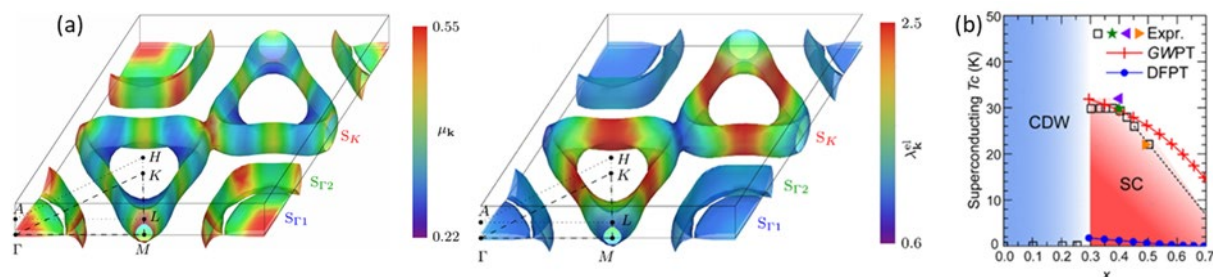
Figure 1. Momentum resolved screened Coulomb interaction and e-ph interaction strength on the FS of 2H-NbS 2 . Reproduced with permission from [5], Copyright 2017 by the American Physical Society. (b) Superconducting phase diagram of \text{Ba}_{1-x}\text{K}_x\text{BiO}_3 . Calculated T_c with \mu^*=0.16 are plotted as red crosses for GWPT and blue dots for DFPT. Experimental data are plotted as squares, star, left-pointing triangle, and right-pointing triangle. Reproduced with permission from [10], Copyright 2019 by the American Physical Society.
