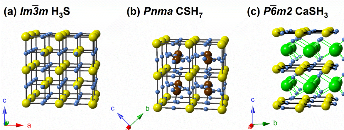
Figure 2. Superconducting high-pressure hydride phases that contain H-S lattices: (a) \text{H}_3\text{S} , (b) \text{CSH}_7 , and (c) \text{CaSH}_3 . Sulfur/hydrogen/carbon/calcium atoms are colored yellow/blue/brown/green. Adapted with permission from J. Phys. Chem. C. 2021 [2]. Copyright (2020) American Chemical Society.
