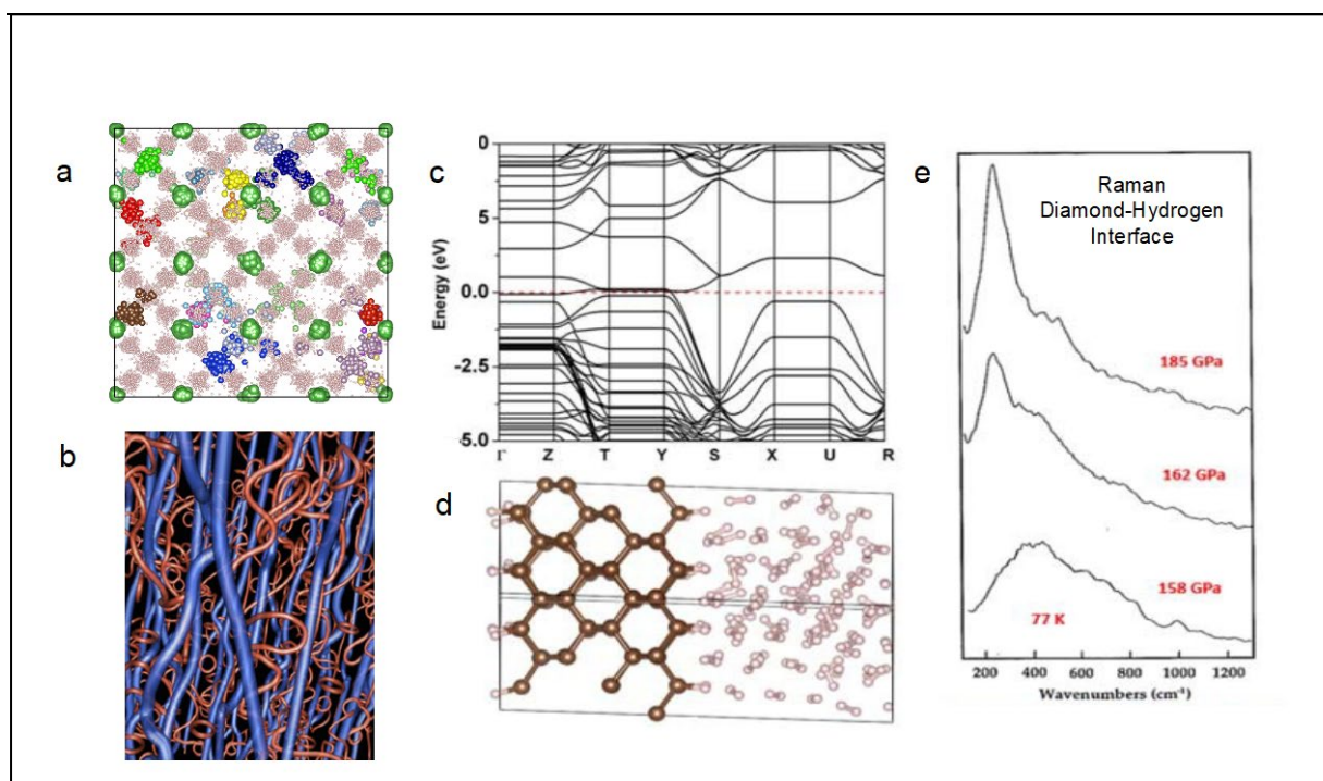
Figure 2. (A) Quantum diffusion and sublattice melting of \text{LaH}_{10} based on path integral molecular dynamics simulations (150 GPa and 800 K). The displacements of the La atoms (green spheres) and H atoms (pink spheres) are shown [from Liu et al., Phys Rev. B 98 , 100102(R) (2018)]; (b) Vortex structure of superconducting superfluid hydrogen [from Babaev et al. Nature 431 , 666-668 (2004)]; (c) Band structure of the 111 diamond surface of diamond covered with a hydrogen monolayer at 350 GPa and (d) molecular dynamics simulations of hydrogen in contact with a 100 diamond surface at 300 GPa (H. Lui et al., unpublished); (e) Raman spectra of the diamond-hydrogen interface near 200 GPa indicating anomalous electronic excitations associated with pressure-induced interfacial electronic transitions [from Hemley and Mao, Phys. Lett. A 163 , 429-434 (1992)].
