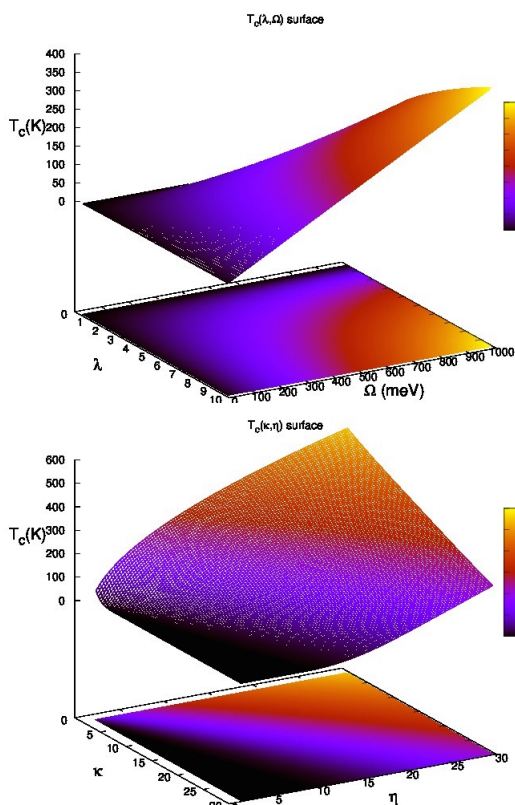
Figure 1. Surface plot and projected heat map of Allen-Dynes’ expression T_c^{AD}(\lambda, \Omega) (origin is at far left) emphasizing the very large range of the arguments. The plot is roughly symmetric, with the maximum lying along ‘diagonal’ with a decrease toward either axis. The implication is that both \lambda and \Omega \propto \Omega^{-2} , which is challenging because \lambda is proportional to \Omega^{-2} . The scale of T_c is normalized to the value of H 3 S at the calculated values of \lambda and \Omega for
