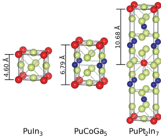
FIG. 1. (Color online) Crystal structures, obtained using VESTA, 6 of some Pu-based compounds. The Pu atoms are colored red, Pt/Co atoms dark blue, and In/Ga atoms light green.
