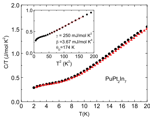
FIG. 3. (Color online) Specific heat data ( C/T ) vs temperature of PuPt 2 In 7 , taken in zero field (black circles) and 6 T (red triangles). Inset shows the data plotted vs T^2 along with a linear fit between 7 and 13 K, from which estimates of the Sommerfeld coefficient and Debye temperature were obtained.
