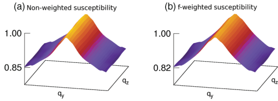
FIG. 10. (Color online) Normalized (a) \chi and (b) \bar{\chi} of PuCoGa 5 in the conventional Brillouin zone for q_x = 0.5 . \mathbf{q} = (0,0,0) are at the corners. Susceptibilities of the other three Pu compounds look qualitatively equivalent.
