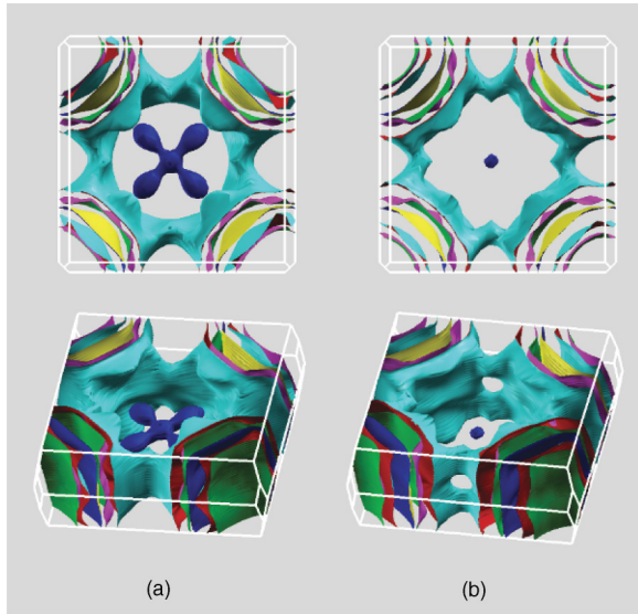
FIG. 7. (Color online) Calculated FSs of (a) PuPt 2 In 7 and (b) PuPt 2 Ga 7 in the GGA + U scheme. \Gamma is located in the center of the unit cell. For clarity, the 3D FSs are reproduced in the bottom figures.
