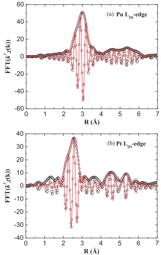
FIG. 2. (Color online) Fast Fourier transformed r -space data (open symbol) and the fit (solid line) for (a) Pu L III edge and (b) Pt L III edge. Both EXAFS data sets were measured at T = 30 K, with a Fourier transformed k range of 3.5–13.5 Å -1 and a Gaussian window of 0.3 Å -1 . The r -space fit range is 2.1–5.4 Å for both edges. Here only the real part, Re, and the amplitude, \sqrt{\text{Re}^2 + \text{Im}^2} , of \text{FFT}[k^3\chi(k)] are plotted.
