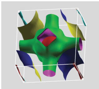
FIG. 8. (Color online) Calculated FSs of PuCoGa 5 in the GGA + U scheme. \Gamma is located in the center of the unit cell.
